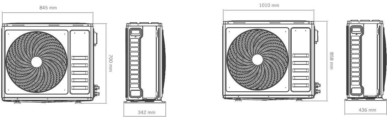
OUTDOOR UNIT · FLOOR-CEILING INVERTER AC 36K BTU
