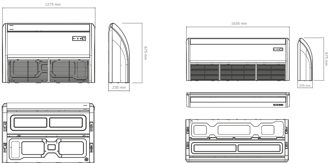
301423 · FLOOR-CEILING INVERTER AC 60K BTU
