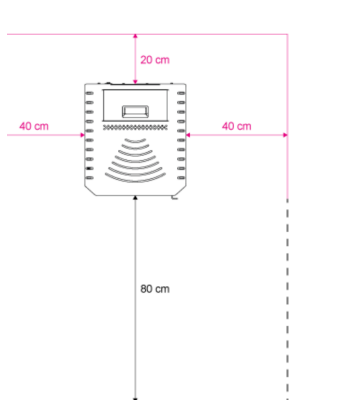
Top view — clearances to observe
