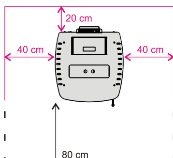
Top view — clearances to observe
