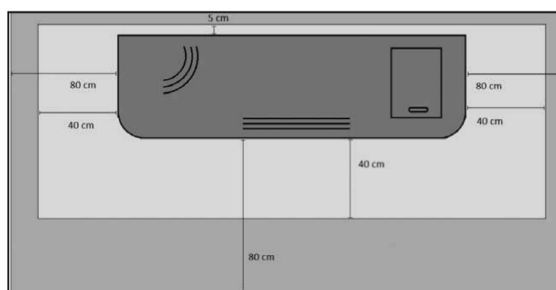
Top view — clearances to observe
